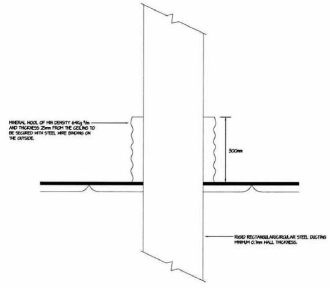
CEILING PENETRATION
